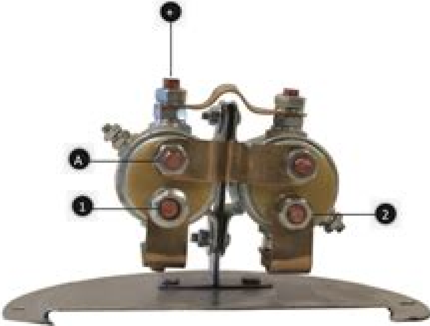
PSS28C ROUND SOLENOID ASSEMBLY
