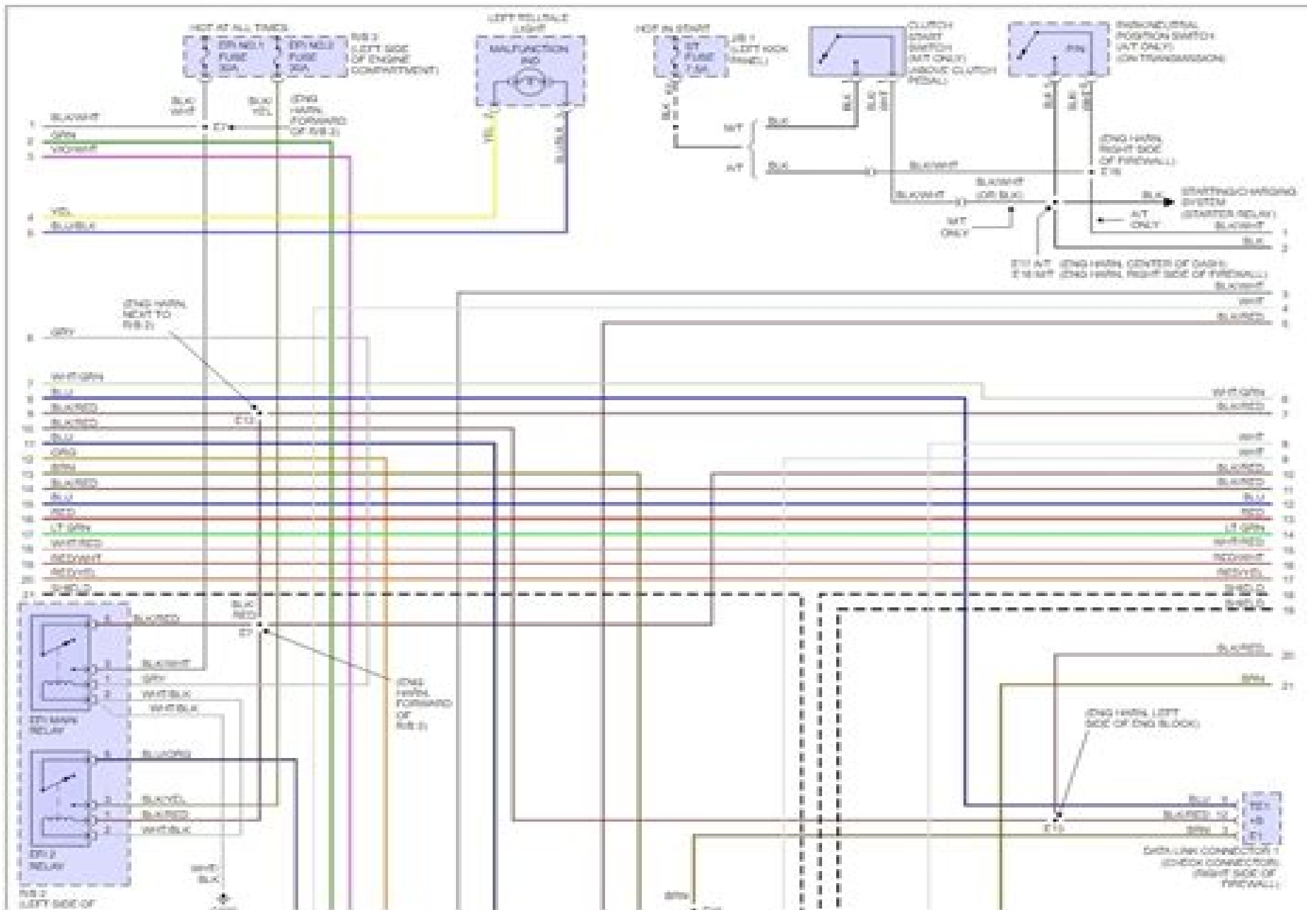
Fig 7: 3.0L Turbo, Engine Performance Circuits (3 of 4)
