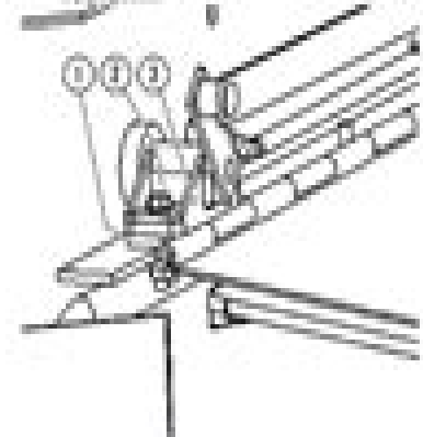
FIGURE 3-4. PILLOW BLOCK INSTALLATION
