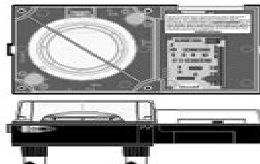
Duct Sensor Housing, Front and Bottom View
