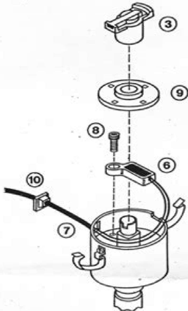
COMPU-FIRE INSTALLATION FIGURE 2
