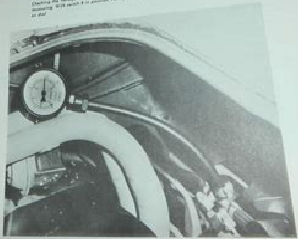
For the hydraulic test the pressure gauge is connected to the fuel line. Gauge as shown after the stop screw has been removed
