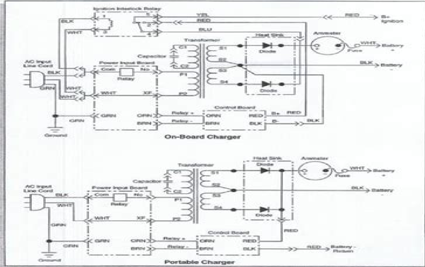
Fig. 5 PowerWise™ Charger Wiring Diagrams
