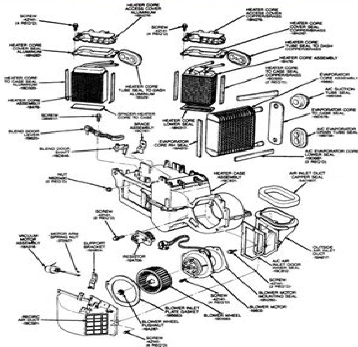
Fig 18 Heater And Evaporator Exploded View
