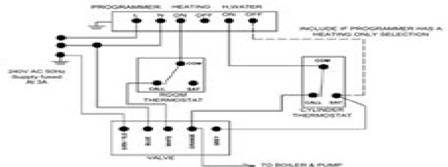
Mid - position Valve Typical circuit showing Programmer, Room and Cylinder Thermostats as control elements
