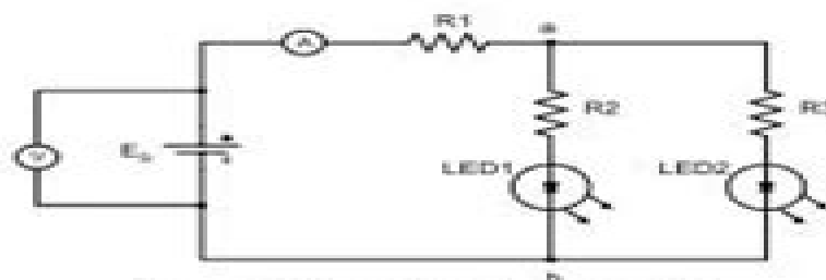
Figure 1: Series-parallel circuit containing LEDs
