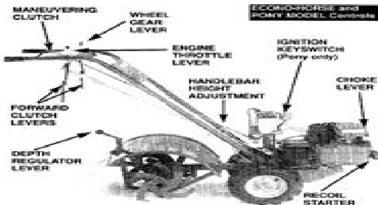
Photo 3-1: Location of controls on the PONY and ECONO-HORSE Models. (Pony Model shown.)
