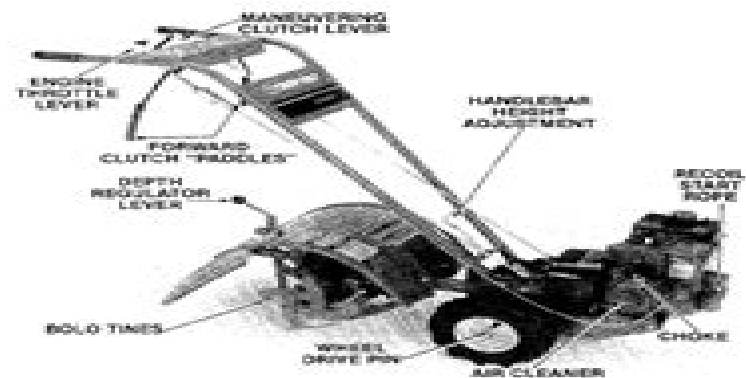
Photo 3-1A: Location of controls on the JUNIOR Model tiller.
