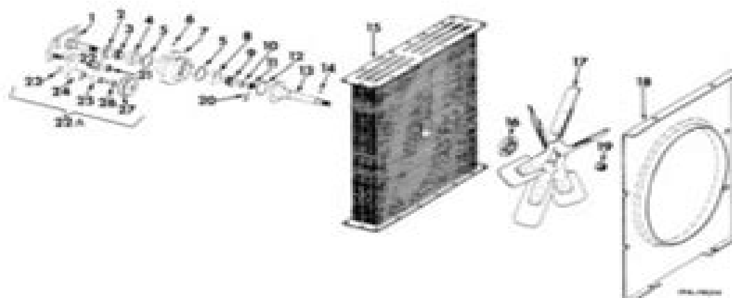
Illustr. 3- Outboard Fan, Radiator, Pulley and Shaft Assembly.
