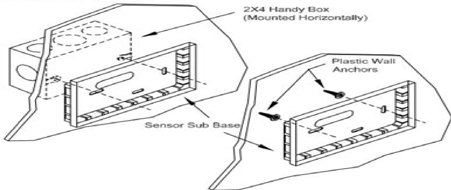
Figure 2 Mounting the Sub Base
