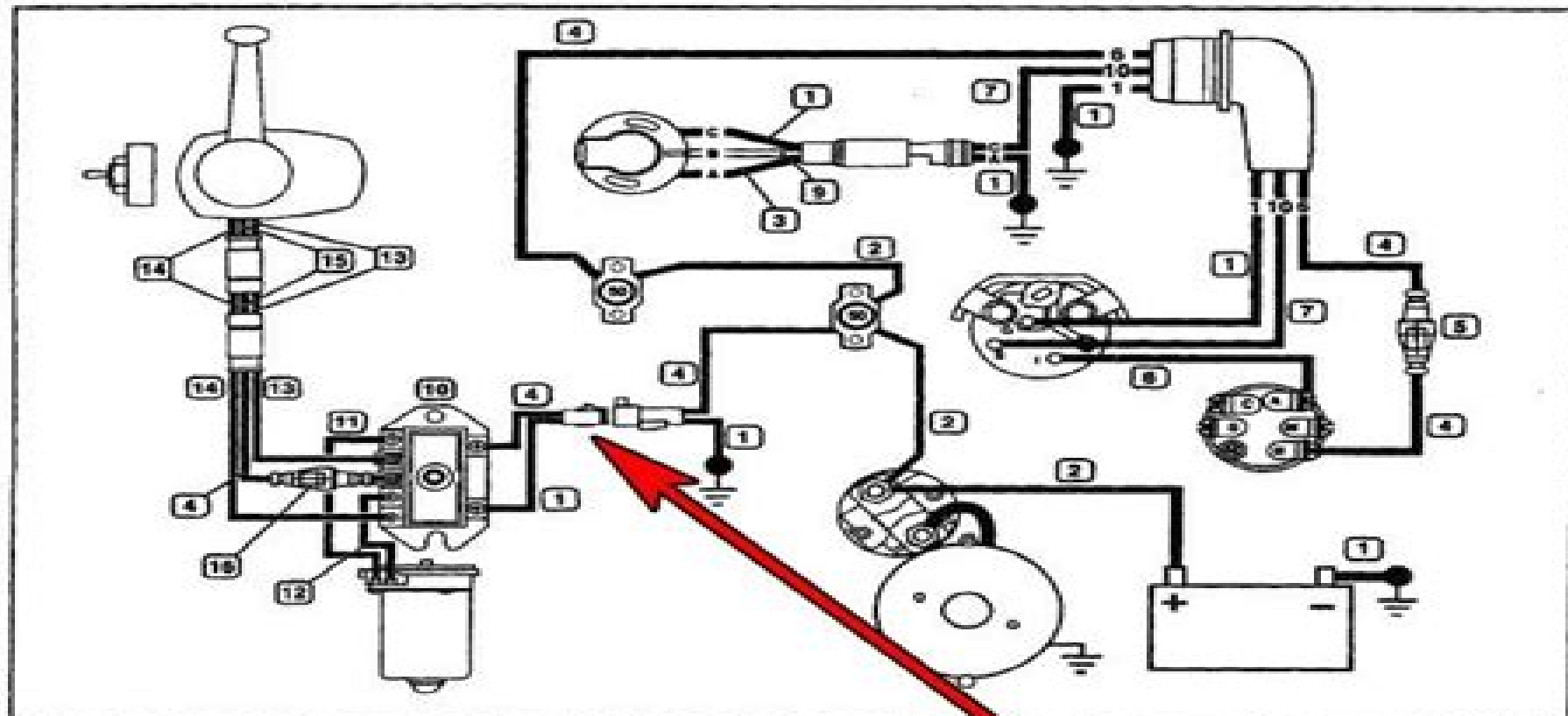
Trim/Tilt Circuit 3.0 GS Models 4.3 GL, GS Models 5.7 GL Models
