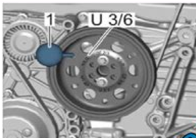
Fig. 2b: Identifying Vibration Damper Marking Courtesy of PORSCHE CARS NORTH AMERICA, INC.
