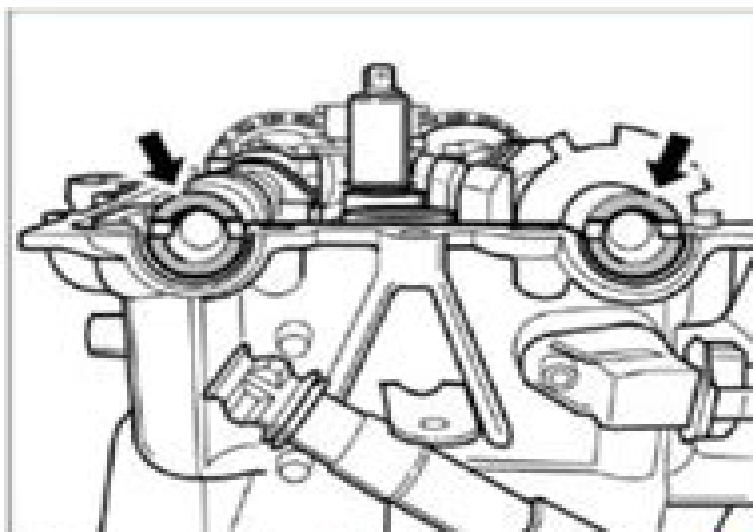
Fig. 39: Side position of camshafts at starting Courtesy of PORSCHE OF NORTH AMERICA, INC.
