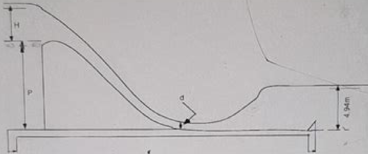
Fig.Q2: Overflow ogee weir with a hydraulic jump formed downstream in the stilling basin.
