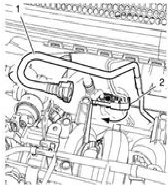
Fig. 32: Fuel Tank Vent Pipe Courtesy of GENERAL MOTORS COMPANY
