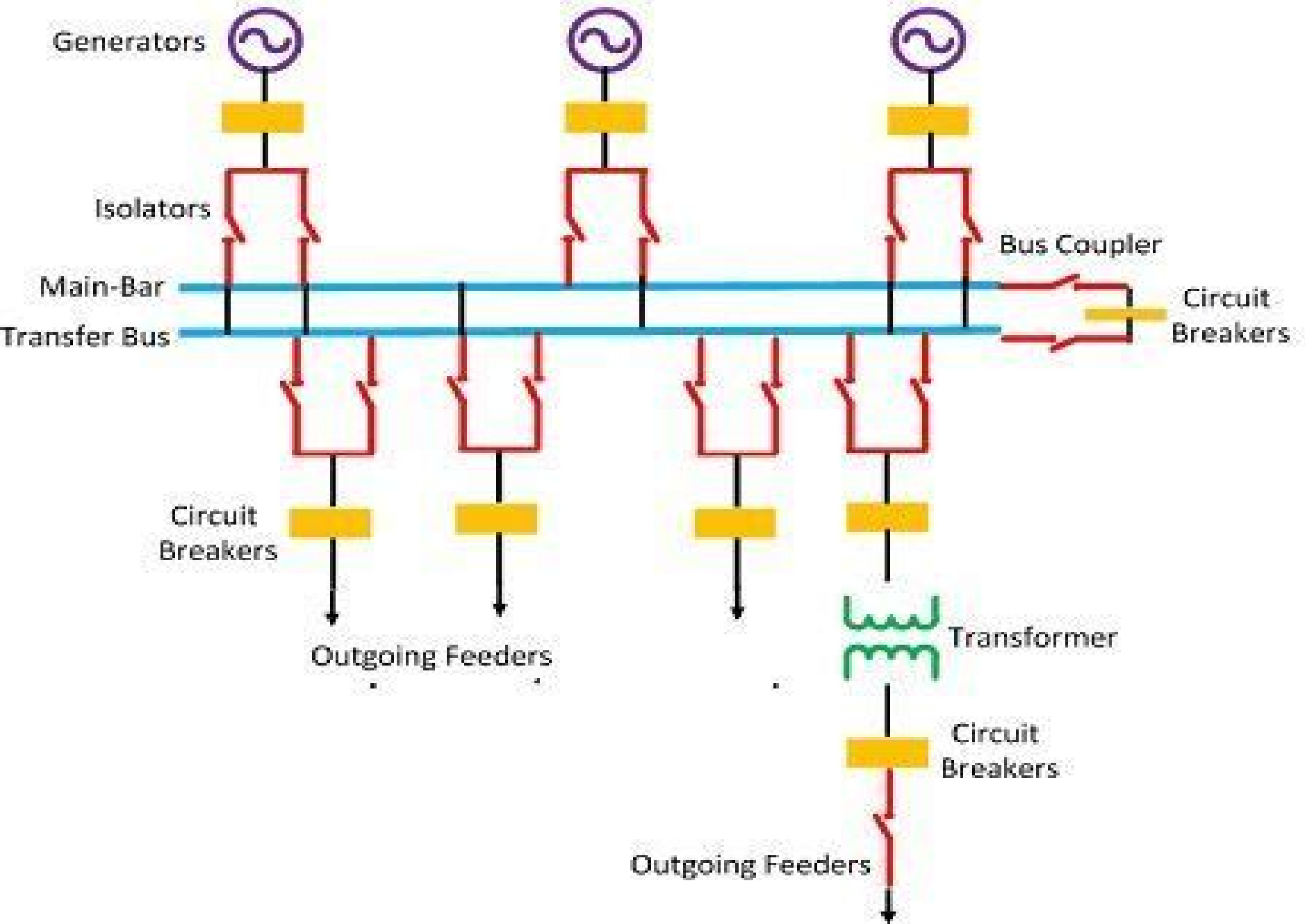
Main And Transfer Bus Arrangement
