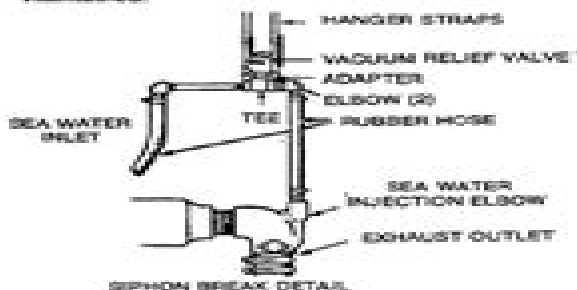
FIGURE 3. TYPICAL INSTALLATION WITH AQUALIFT MUFFLER
