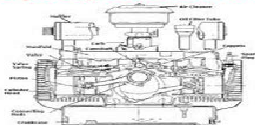
TYPICAL ENGINE (CROSS SECTION)
