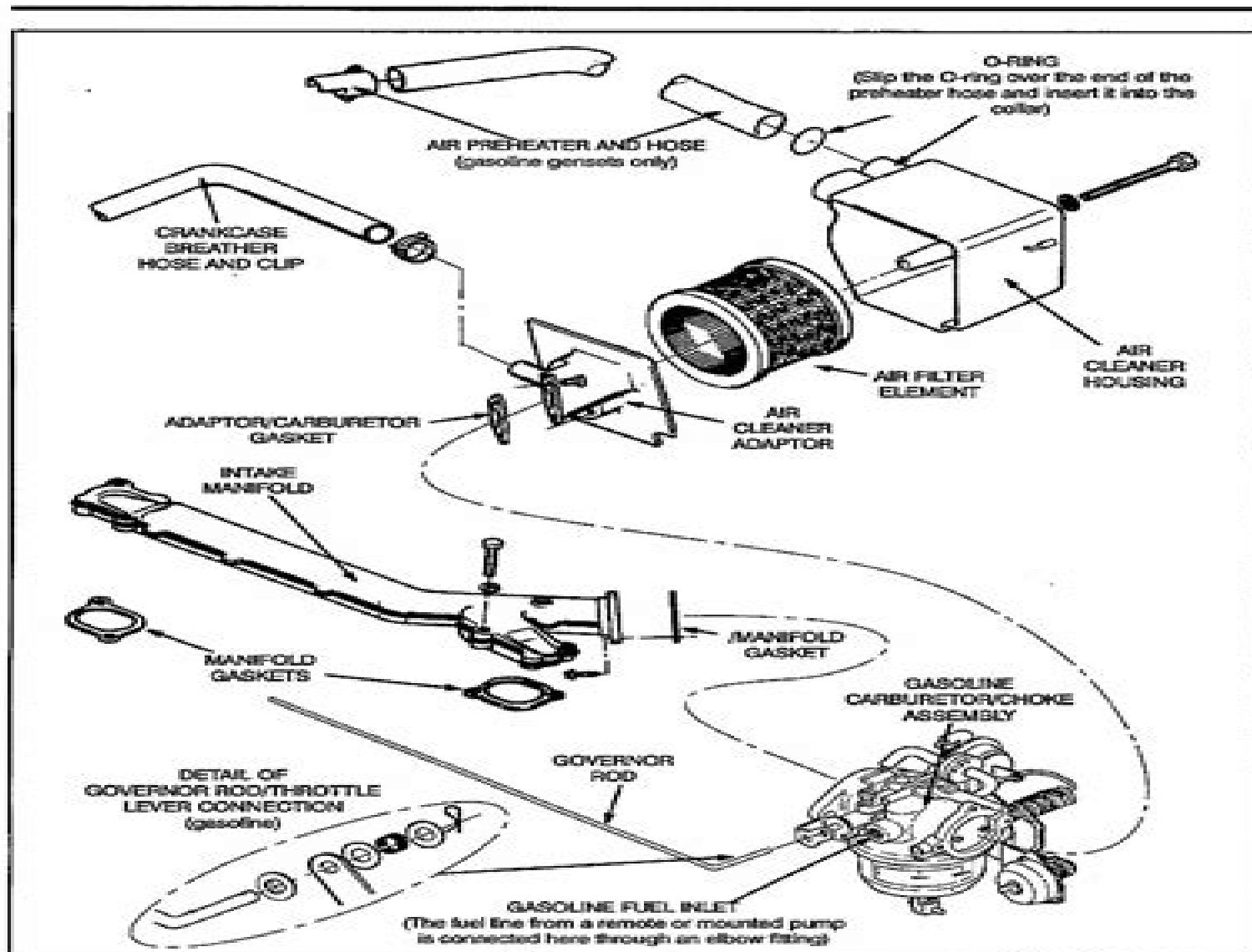
FIGURE S-1. TYPICAL FUEL SYSTEM
