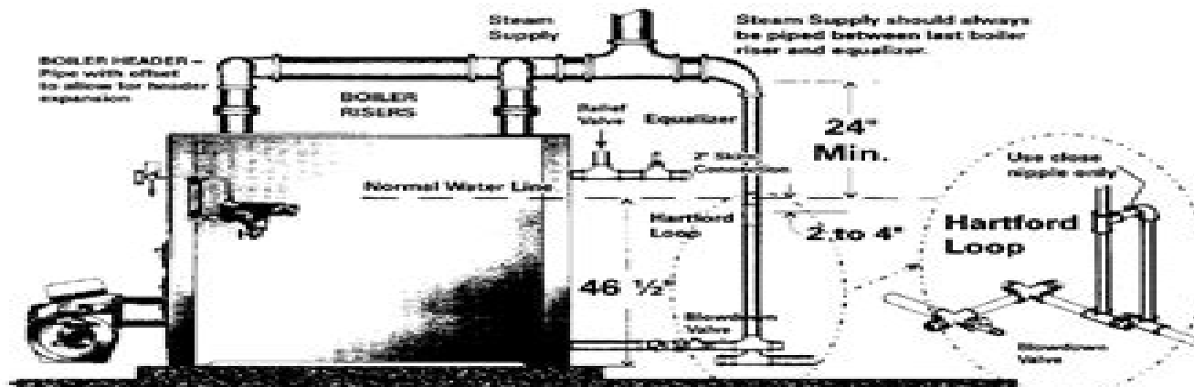
Figure 19: Supply and Return Positions, Skim Piping, Hartford Loop
