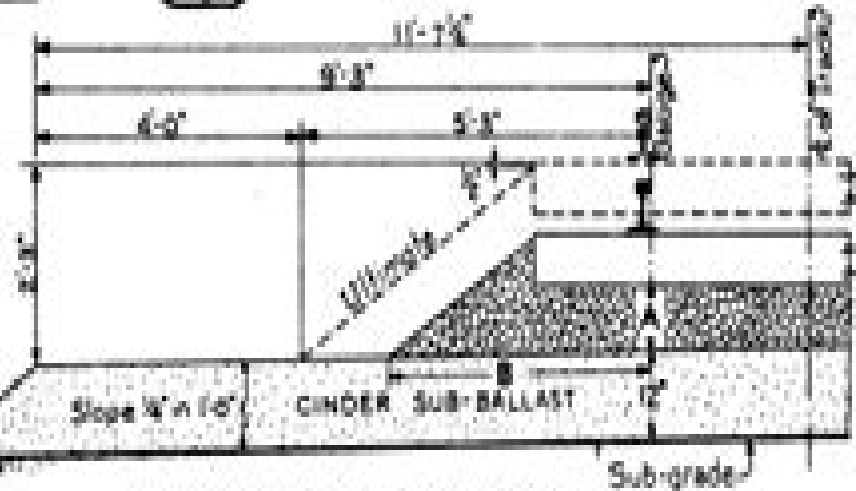
SECTION OF ROADWAY ON FILLS.
