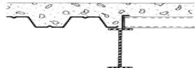
CELL CLOSURE
