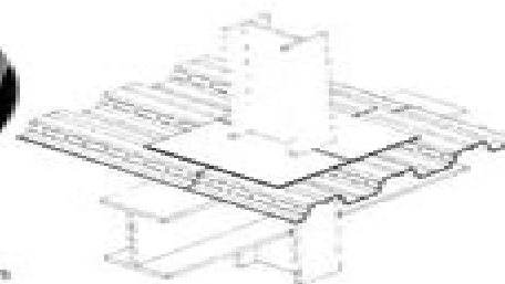
COLUMN CLOSURE
