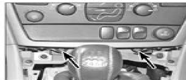
10.9a Undo the 2 Torx screws (arrowed) ...
