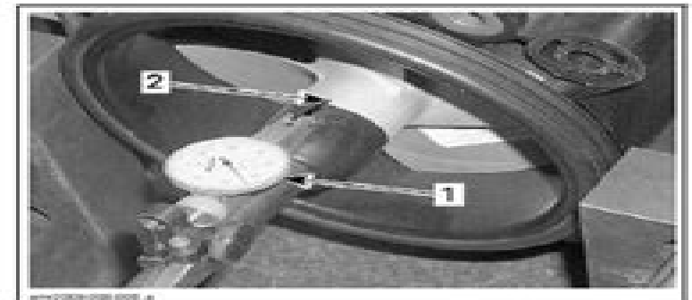
TYPICAL — MEASURING IMPELLER SHAFT RADIAL PLAY 1. Dial gauge 2. Measure close to impeller hub end
