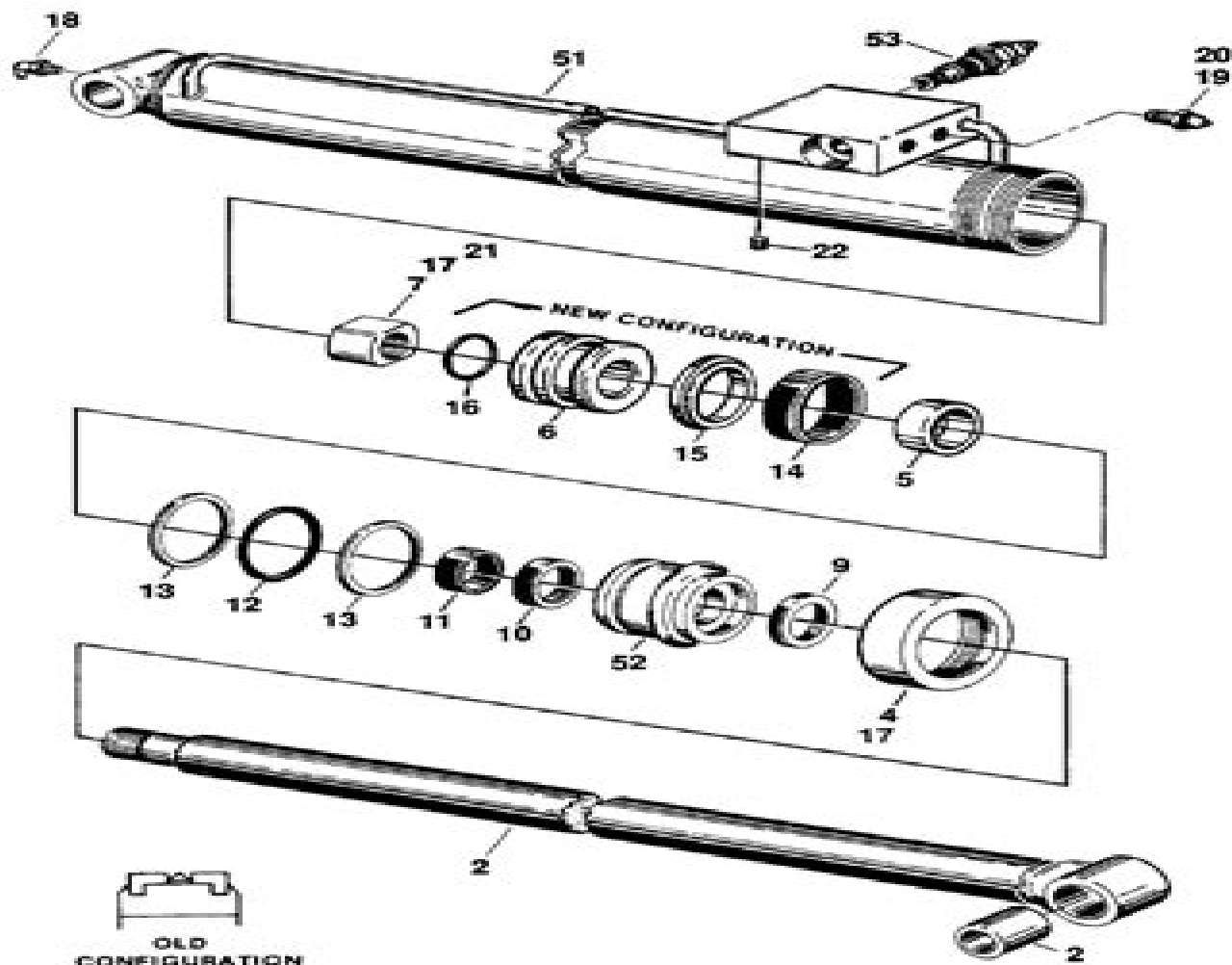
FIGURE 5-7. PLATFORM LEVEL CYLINDER ASSEMBLIES (BUILT PRIOR TO JANUARY 1987)
