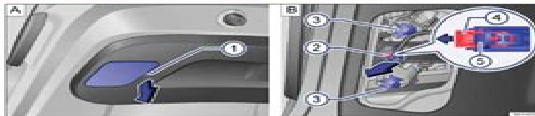
Fig. 221 A: In the luggage compartment lid: Removing the taillight cover. B: Removing the taillight assembly.
