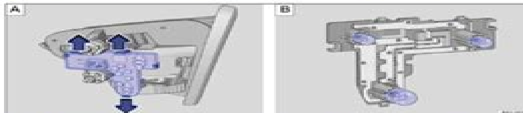
Fig. 222 A: Taillight assembly: removing the bulb socket assembly. B: Removing the light bulbs.
