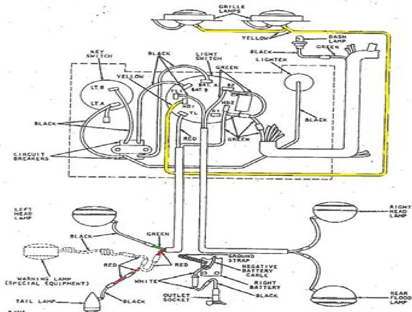
Fig. 200-45-6—Lamp Wiring Diagram for Diesel Tractors
