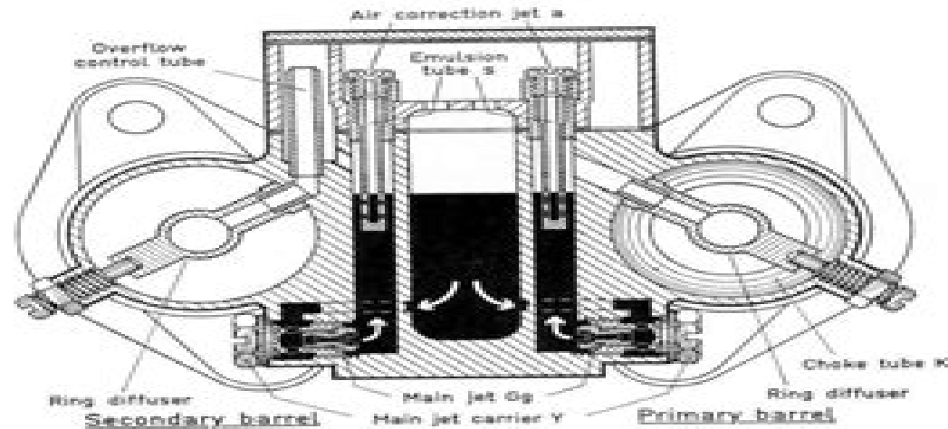
Fig. 27 Jet assembly of the 44 PWH carburetor
