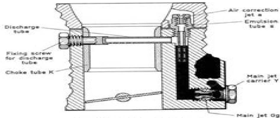
Fig. 28 Jet assembly of the 48 PII carburetor
