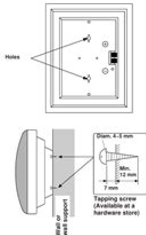
Upright configuration
