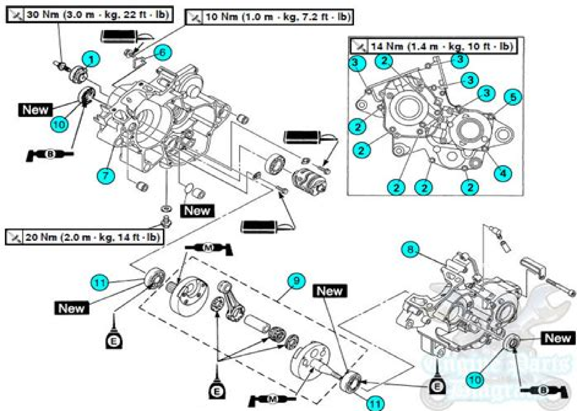
Yamaha YZ125 Crankcase and Crankshaft Parts Diagram
