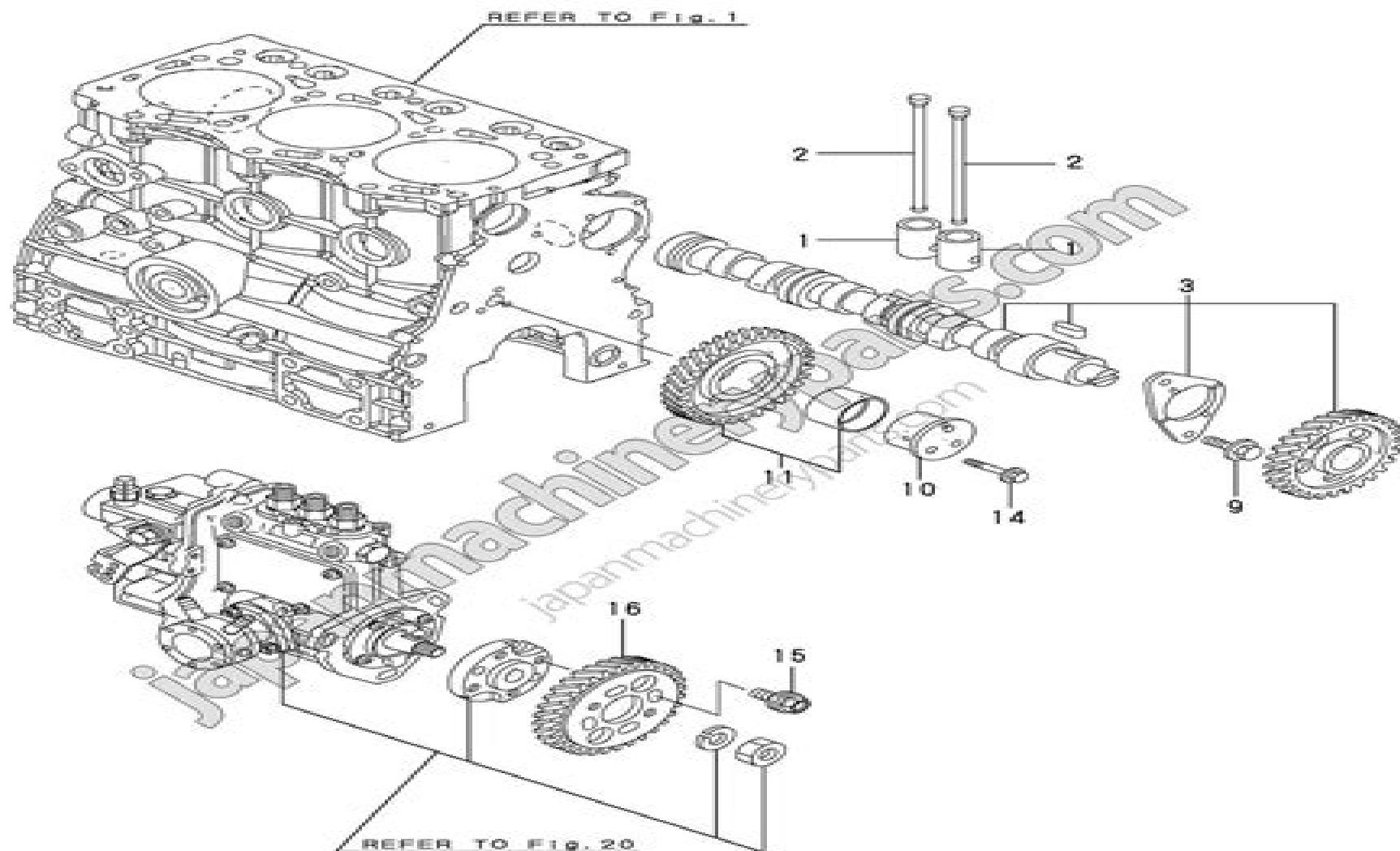
Fig.9. CAMSHAFT & DRIVING GEAR
