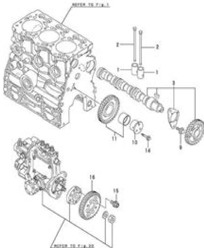
Fig.9. CAMSHAFT & DRIVING GEAR
