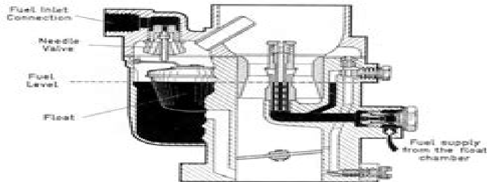
Fig. 6 The Float System
