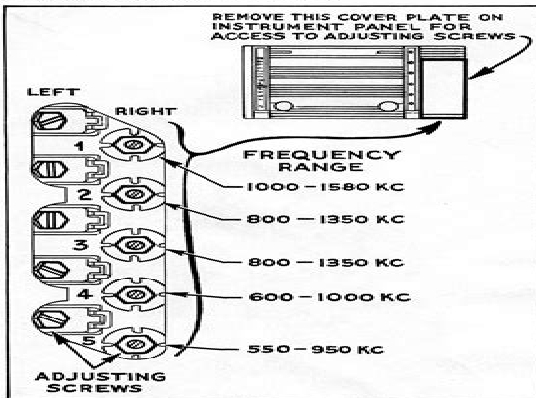
Figure 5 ADJUSTING SCREWS AND FREQUENCY RANGE
