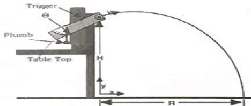
FIGURE 1: Projectile Motion
