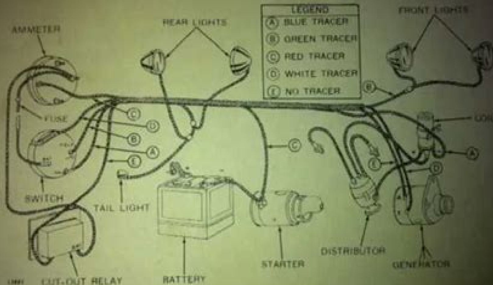
Figure 200-10-9—Wiring Harness
