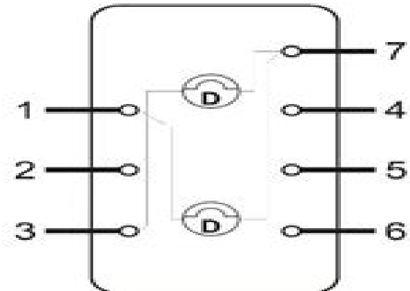
LAMP DIAGRAM
