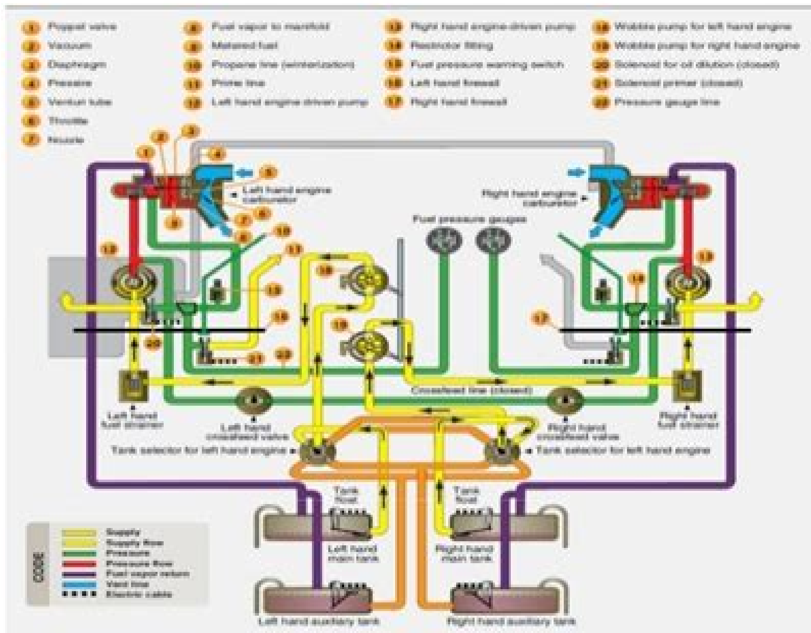
Figure 14-10. DC-3 fuel system.
