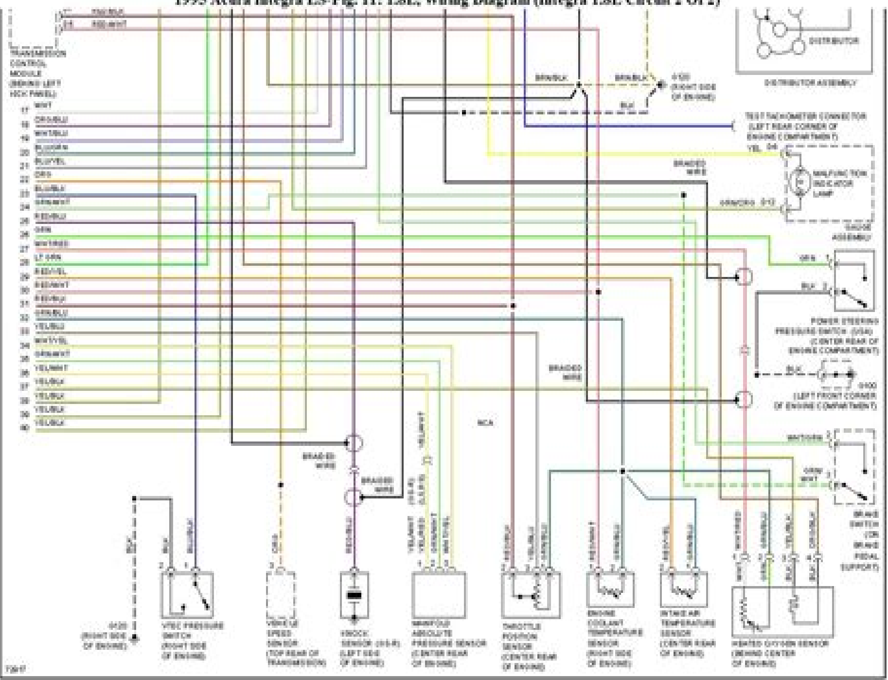
1995 Acura Integra LS Fig. 11: 1.8L, Wiring Diagram (Integra 1.8L Circuit 2 Of 2)
