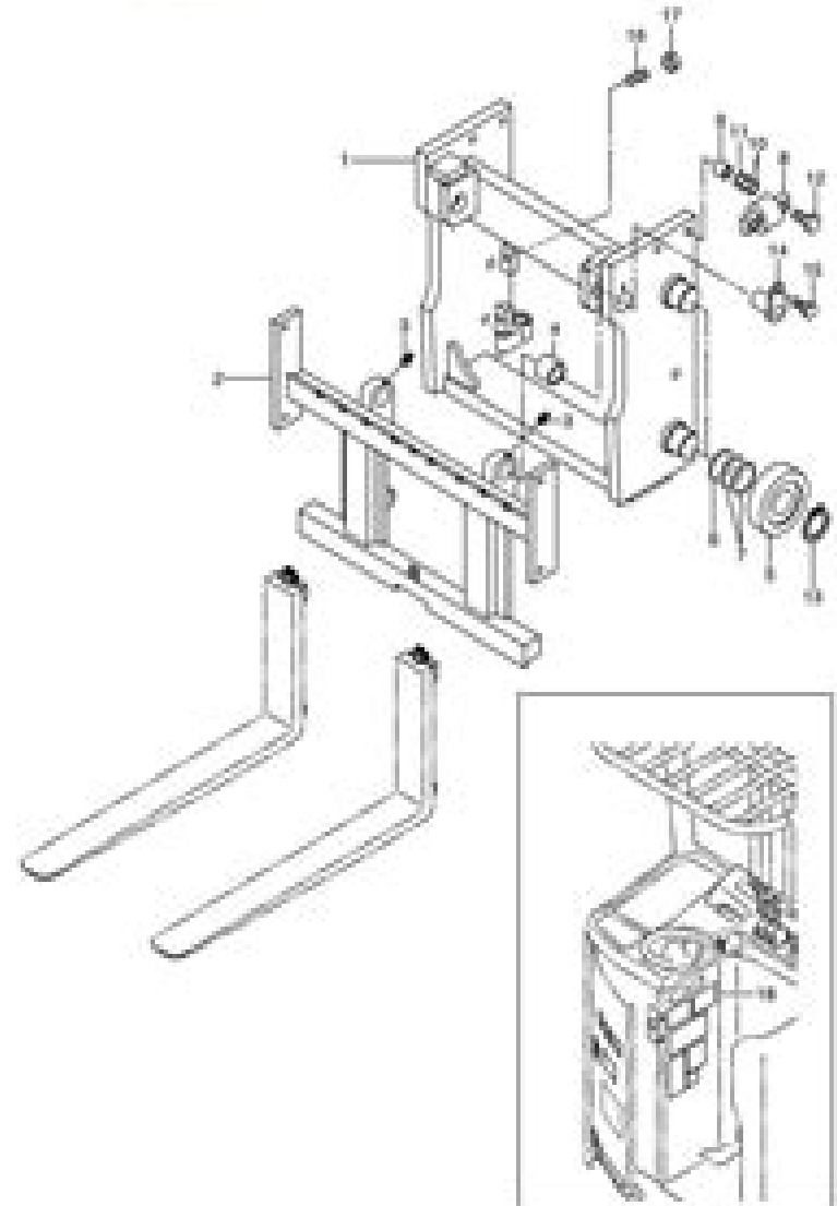
FIG. 99 LIFT BRACKET (LB) (VM750) 5217 5011
