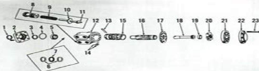
Fig. 9 - Exploded view of steering control assembly. Centering springs (14) are installed in two groups of three springs with arch in each group back-to-back.
