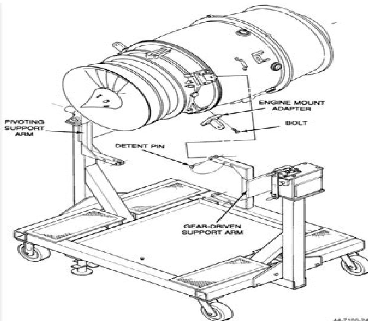
Fig. 401 Engine in Build Stand - Removal/Installation
