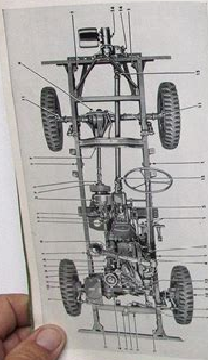
FIG. 1—MURRAY C-14 AND C-15 ALTERNATION CHASSIS ALL DIMENSIONS IN INCHES UNLESS OTHERWISE SPECIFIED
