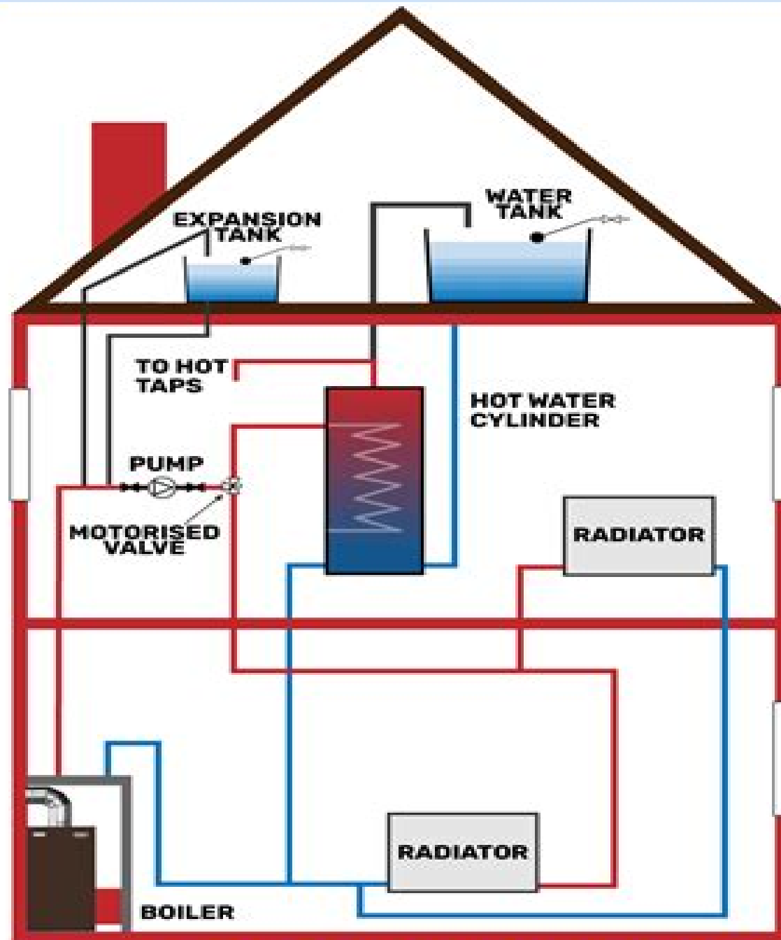
FULLY PUMPED OPEN VENTED SYSTEM
