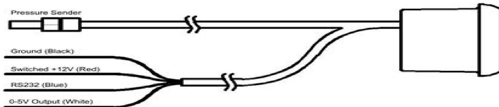
Figure 1. Connection Diagram
