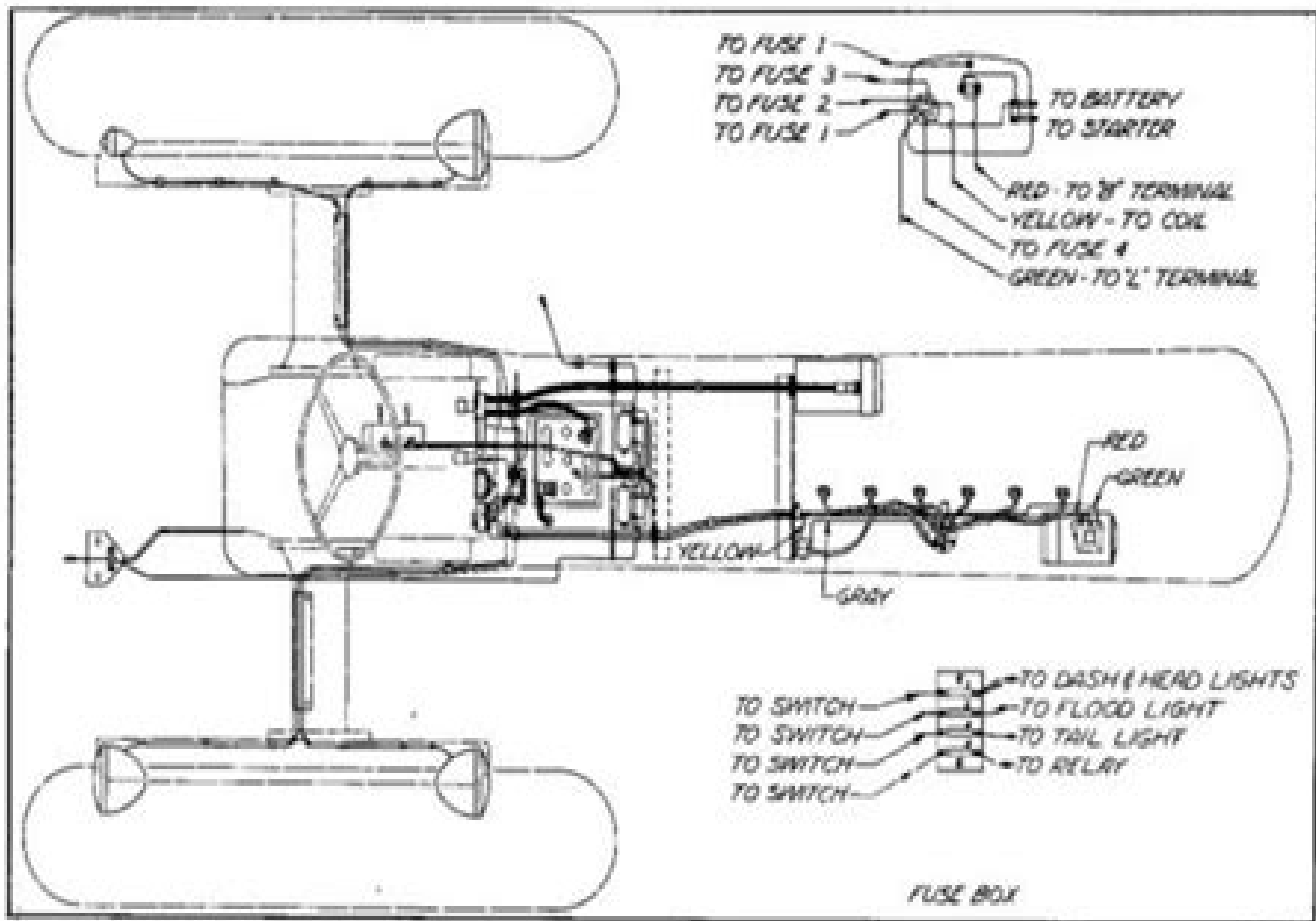
Figure 4-2 Fleetline 77, 88 HC And LPG 6-Volt Wiring Diagram
