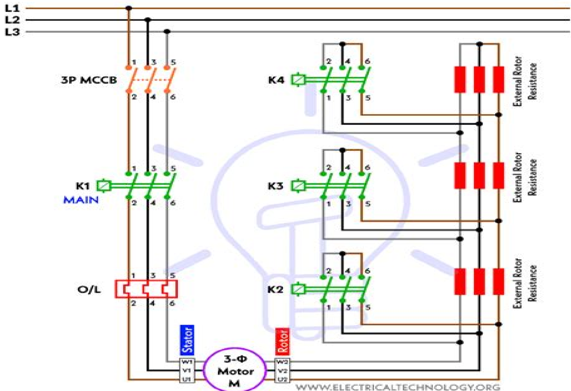
3-Phase Slip Ring Induction Motor
